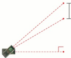
Pythagoras function
